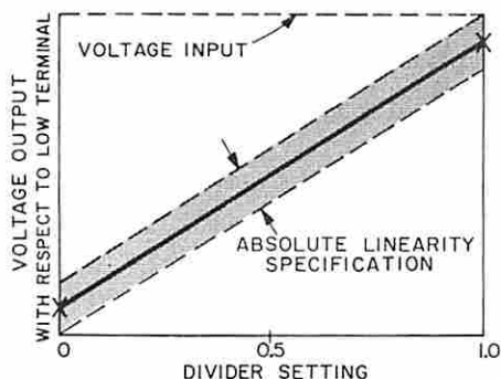
Figure 3-2. Exaggerated illustration of absolute linearity of a Type 1455.
