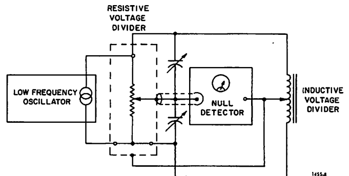
Figure 2-6. An ac null circuit for linearity test of an inductive voltage divider, using a resistive (Type 1455) voltage divider.
