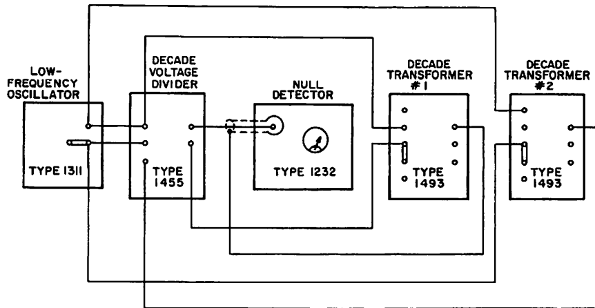
Figure 4-1. Linearity test of a Type 1455 Decade Voltage Divider using a General Radio oscillator, null detector, and two (Type 1493) Precision Decade Transformers.
