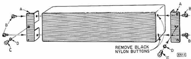
Figure 2-1. Relay-rack installation of a Type 1455 Decade Voltage Divider.
